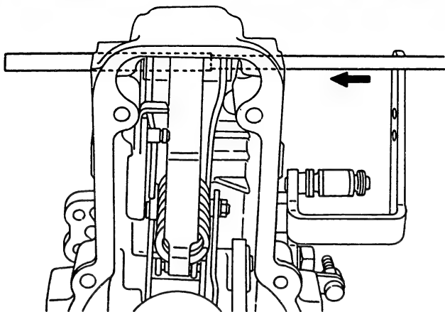
Fig. 35 Drawing out tension lever shaft
